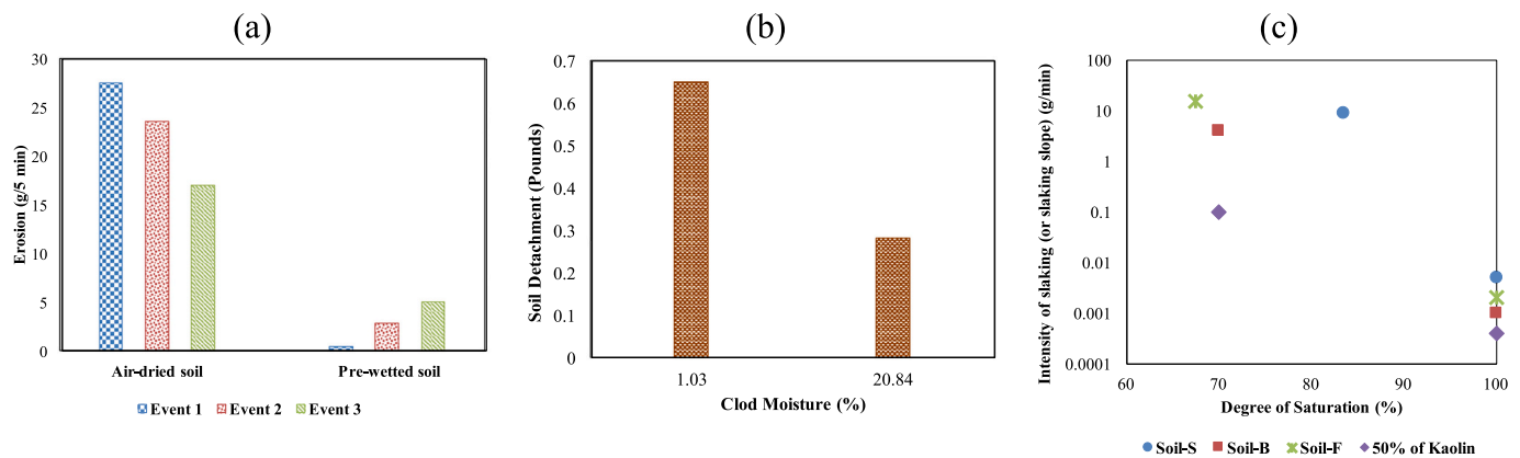
Fig. 1. (a) The change in erosion between initially air-dry and pre-wetted Solono soil for three consecutive rainfall events 24 h and 7 days apart as reported in Lé Bissonnais and Singer (1992) , (b) Effect of moisture on soil detachment based on Lyles et al. (1974) , (c) Changes in the intensity of slaking with degree of saturation in non-dispersive soils, as reported in Lim (2006) .
